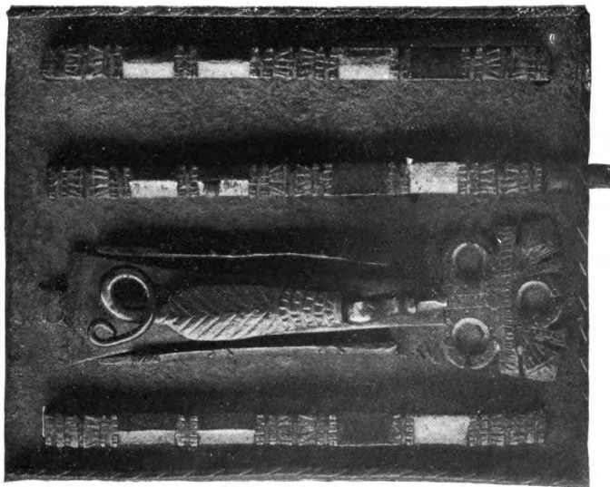
FIG. 61.—Chest-lock. French, late 15th century. Victoria and Albert Museum. Lock-plate, 8 \frac{1}{2} in. long ; 6 \frac{1}{4} in. wide. No. 566-1895.
