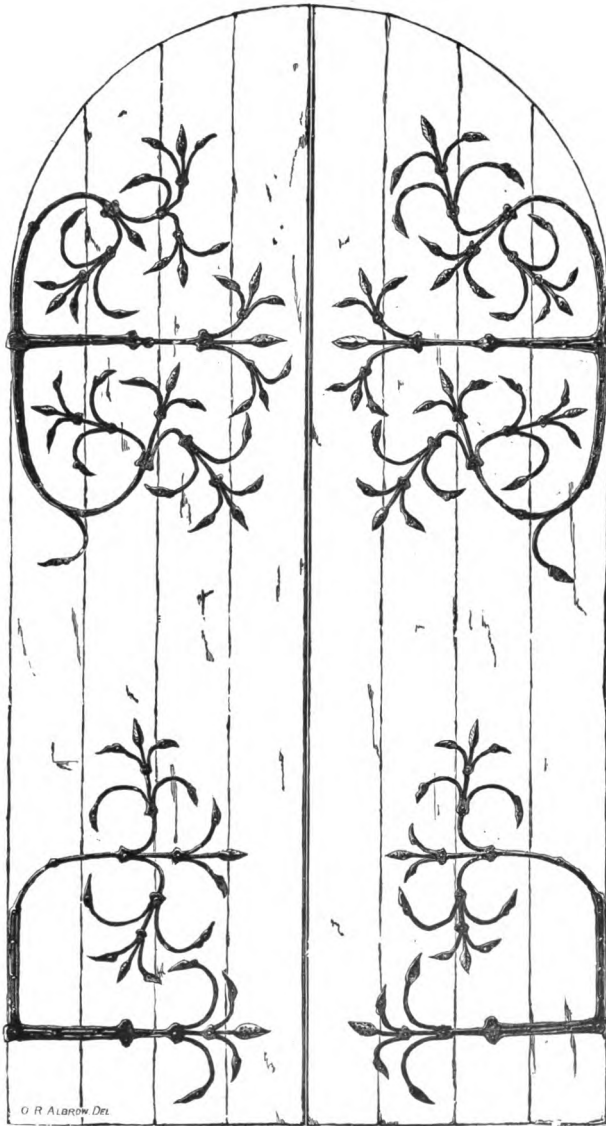
FIG. 34 —Hinges at Market Deeping Church.
